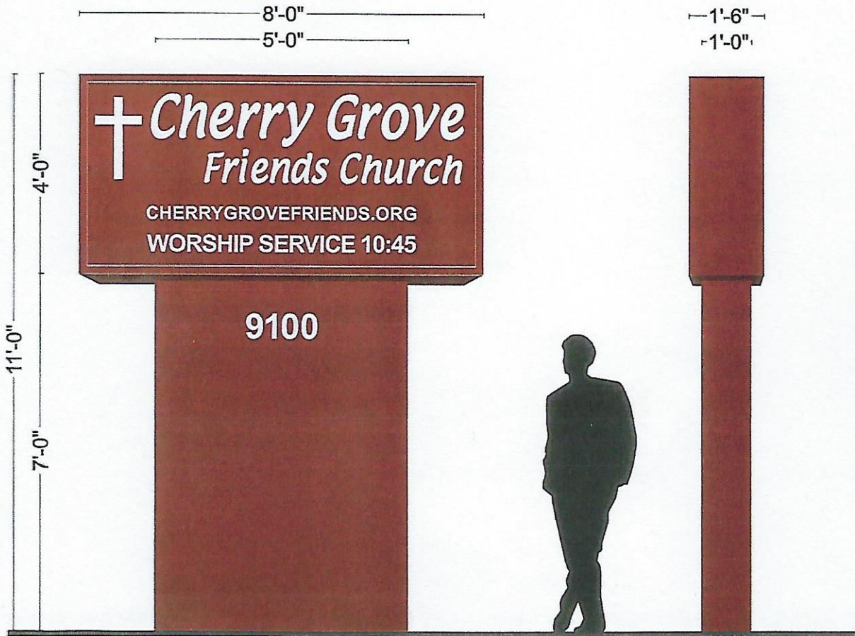
END VIEW CONFIRM DEPTHS
